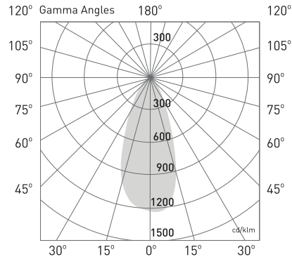
Beam Angle: 50°
